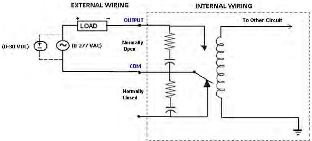
Relay Output Wiring
